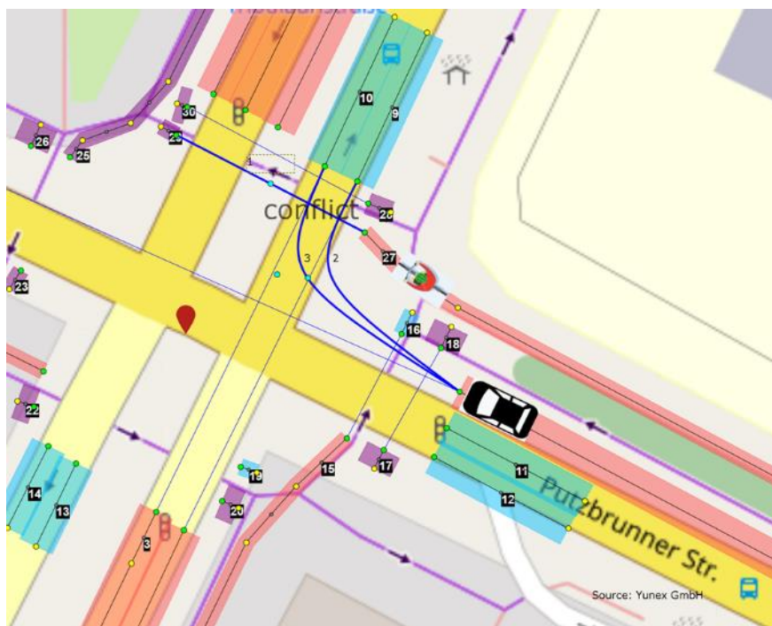
Figure 53: Example for a conflict within the conflict zone that can be addressed precisely by using the connection's Id (connection 2 and 3) instead of absolute lane numbering. Connection-Ids 2 and 3 are unique within the conflict zone and all receivers can evaluate quickly if they cross or came close to those connections or not. (Provided by Yunex GmbH in the scope of C2C-CC's WorkItem D0025)
