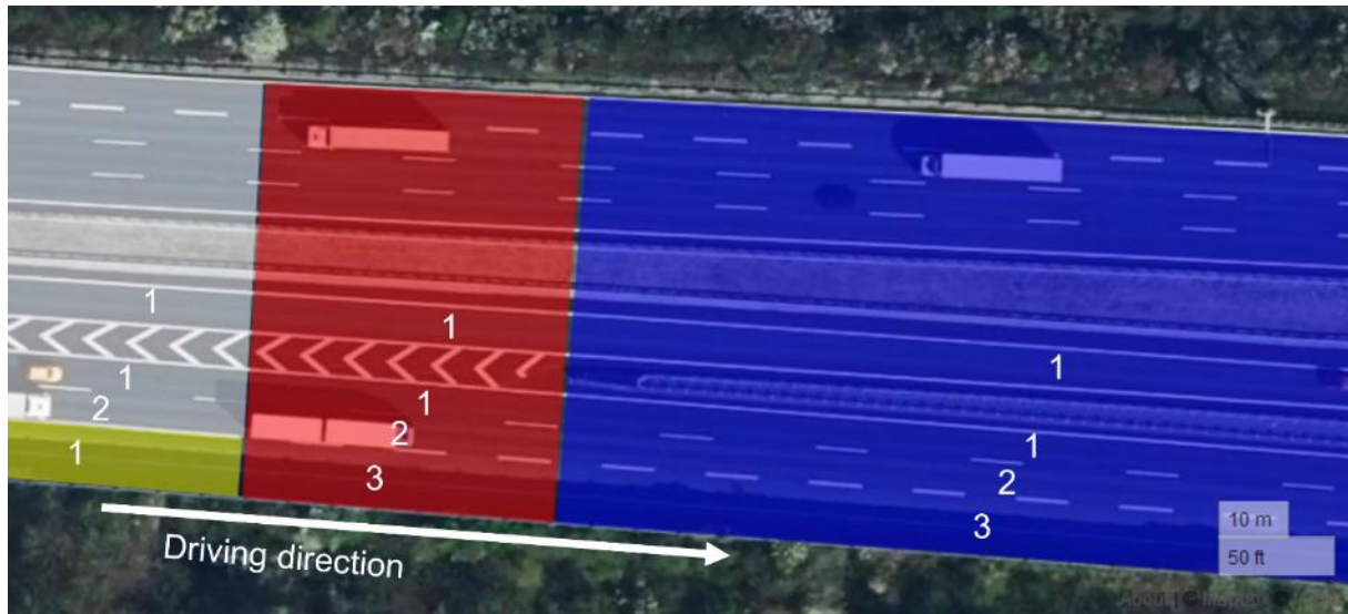
Figure 36: ADASIS-road segments for the scenario in clause 3.2 (where the lanes are separated from each other) with the expected ETSI LanePositions . (Source: created using https://geojson.io © Mapbox (see: https://www.mapbox.com/about/maps/ ) © Maxar (see: https://www.maxar.com/ ))
