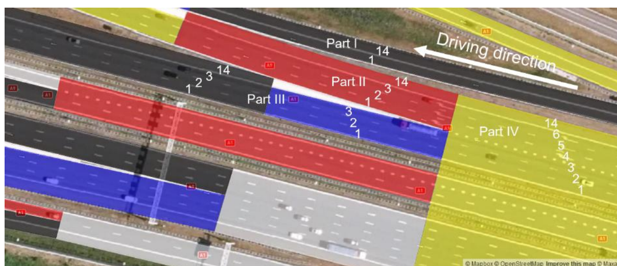
Figure 43: ADASIS-road segments for the eastern end of scenario in clause 3.3 (where the exit lane starts) with the expected ETSI LanePositions. (Source: created using https://geojson.io © Mapbox (see: https://www.mapbox.com/about/maps/ ) © Maxar (see: https://www.maxar.com/ ))
