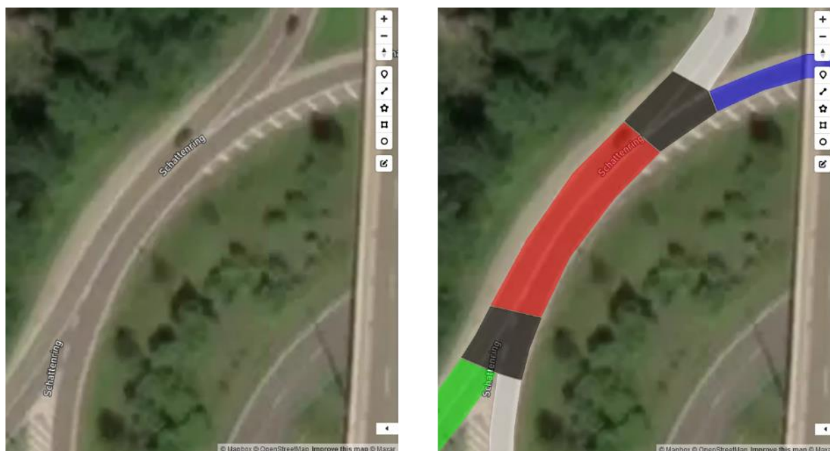
Figure 58: Merging to and diverging from the roundabout with a two-lane road, resulting in short three-lane segments. The original image on the left and the ADASIS-road segments with the expected ETSI LanePositions on the right. (Source: created using https://geojson.io © Mapbox (see: https://www.mapbox.com/about/maps/ ) © Maxar (see: https://www.maxar.com/ ))
