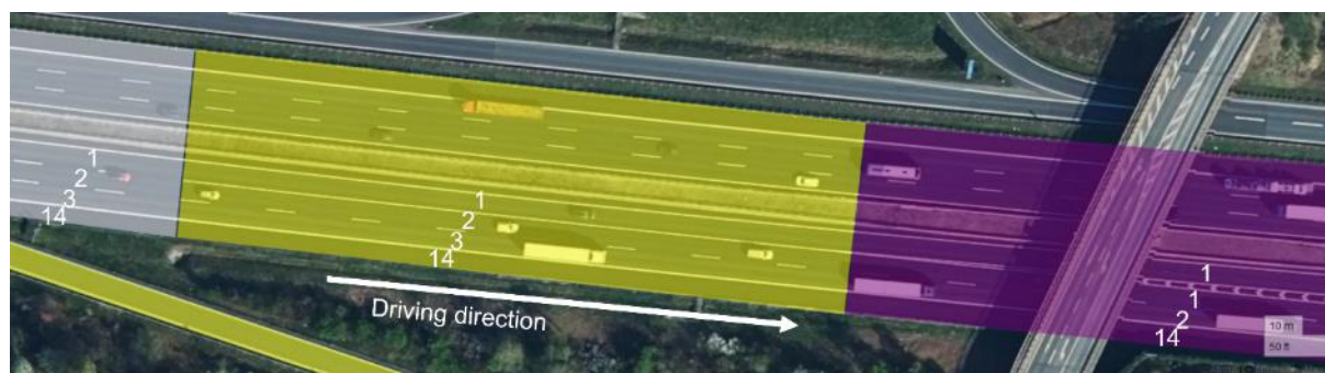
Figure 34: ADASIS-road segments for the scenario in clause 3.2 (where the lanes diverge) with the expected ETSI LanePositions. (Source: created using https://geojson.io © Mapbox (see: https://www.mapbox.com/about/maps/ ) © Maxar (see: https://www.maxar.com/ ))
