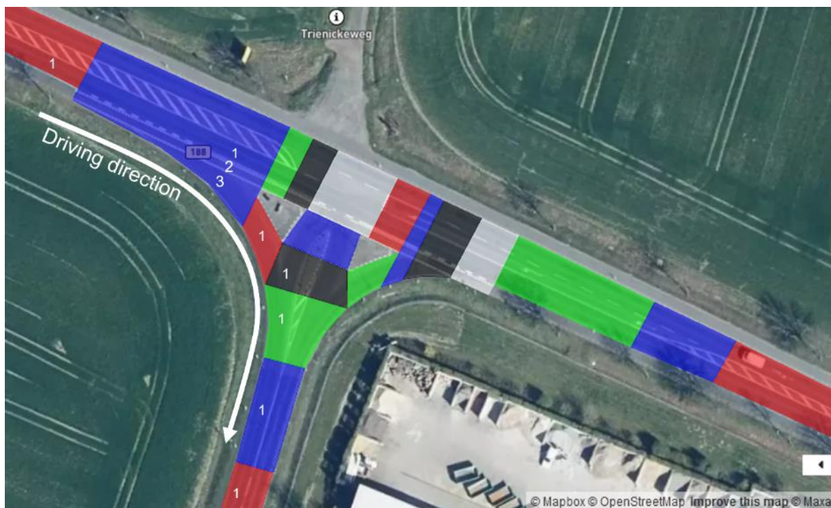
Figure 60: ADASIS-road segments for the scenario in clause 3.12 with the expected ETSI LanePositions for vehicles turning right. (Source: created using https://geojson.io © Mapbox (see: https://www.mapbox.com/about/maps/ ) © Maxar (see: https://www.maxar.com/ ))
