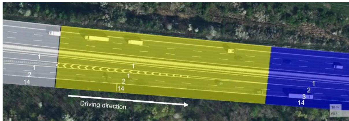
Figure 37: ADASIS-road segments for the scenario in clause 3.2 (where the lanes merge) with the expected ETSI LanePositions. (Source: created using https://geojson.io © Mapbox (see: https://www.mapbox.com/about/maps/ ) © Maxar (see: https://www.maxar.com/ ))
