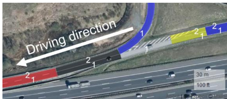
Figure 33: ADASIS-road segments for the scenario in clause 3.1 (where two lanes merge on an exit ramp) with the expected ETSI LanePositions. (Source: created using https://geojson.io © Mapbox (see: https://www.mapbox.com/about/maps/ ) © Maxar (see: https://www.maxar.com/ ))
