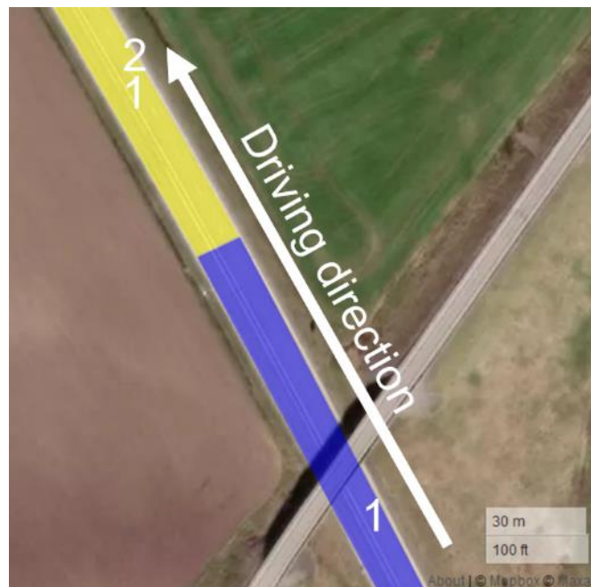
Figure 46: ADASIS-road segments for the scenario in clause 3.5 with the expected ETSI LanePositions. (Source: created using https://geojson.io © Mapbox (see: https://www.mapbox.com/about/maps/ ) © Maxar (see: https://www.maxar.com/ ))
