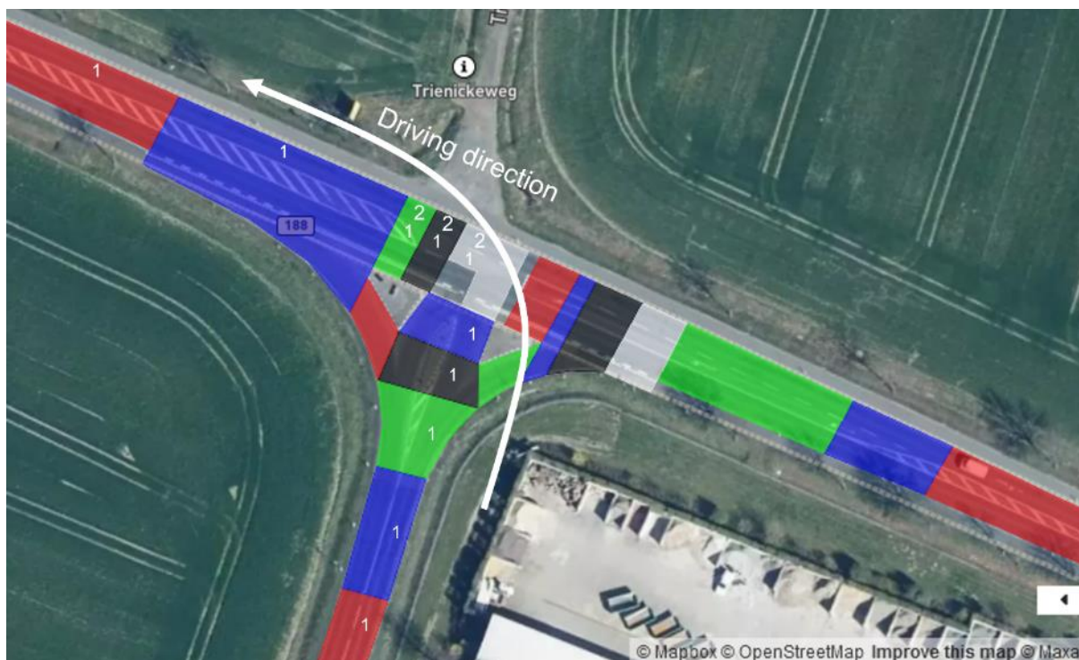
Figure 61: ADASIS-road segments for the scenario in clause 3.12 with the expected ETSI LanePositions for vehicles approaching from the south and turning left. (Source: created using https://geojson.io © Mapbox (see: https://www.mapbox.com/about/maps/ ) © Maxar (see: https://www.maxar.com/ ))
