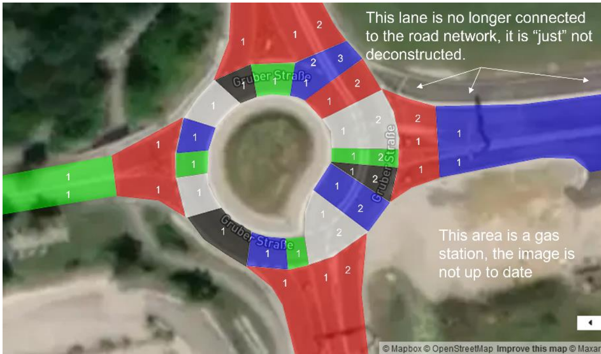
Figure 56: ADASIS-road segments for the scenario in clause 3.10 with the expected ETSI LanePositions . (Source: created using https://geojson.io © Mapbox (see: https://www.mapbox.com/about/maps/ ) © Maxar (see: https://www.maxar.com/ ) )
