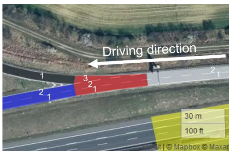
Figure 32: ADASIS-road segments for the scenario in clause 3.1 (where the exit ramp splits) with the expected ETSI LanePositions. (Source: created using https://geojson.io © Mapbox (see: https://www.mapbox.com/about/maps/ ) © Maxar (see: https://www.maxar.com/ ))
