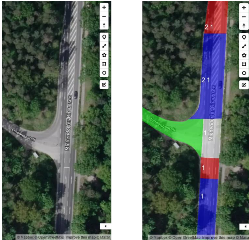
Figure 63: ADASIS-road segments for the scenario in clause 3.13 with the expected ETSI LanePositions. (Source: created using https://geojson.io © Mapbox (see: https://www.mapbox.com/about/maps/ ) © Maxar (see: https://www.maxar.com/ ))
