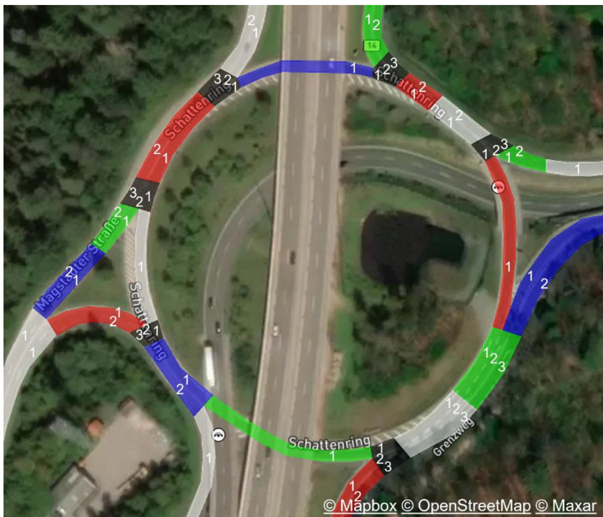
Figure 57: ADASIS-road segments for the scenario in clause 3.11 with the expected ETSI LanePositions . (Source: created using https://geojson.io © Mapbox (see: https://www.mapbox.com/about/maps/ ) © Maxar (see: https://www.maxar.com/ ))
