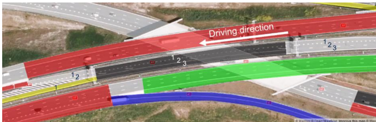
Figure 40: ADASIS-road segments and ADASIS lane numbering for the central crossing of scenario in clause 3.3 (where the motorways crosses each other). (Source: created using https://geojson.io © Mapbox (see: https://www.mapbox.com/about/maps/ ) © Maxar (see: https://www.maxar.com/ ))
