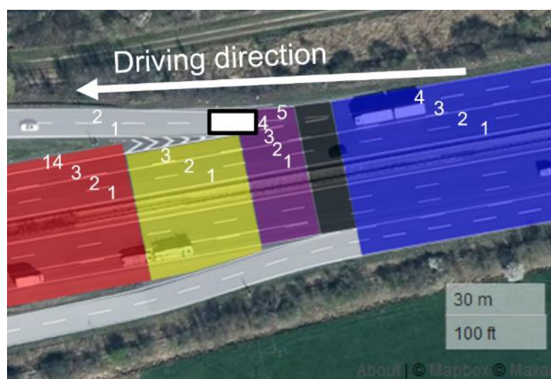
Figure 64: ADASIS-road segments for the scenario in clause 3.1 and the issue with occupation (white box with black border) when extending of road segments. (Source: created using https://geojson.io © Mapbox (see: https://www.mapbox.com/about/maps/ ) © Maxar (see: https://www.maxar.com/ ))
