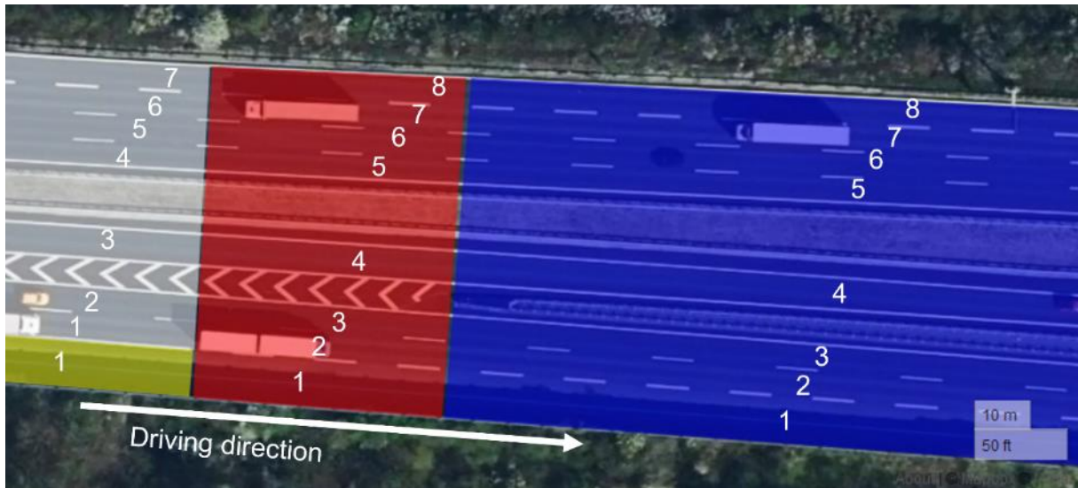
Figure 35: ADASIS-road segments for the scenario in clause 3.2 (where the lanes are separated from each other) with the ADASIS lane numbering. (Source: created using https://geojson.io © Mapbox (see: https://www.mapbox.com/about/maps/ ) © Maxar (see: https://www.maxar.com/ ))
