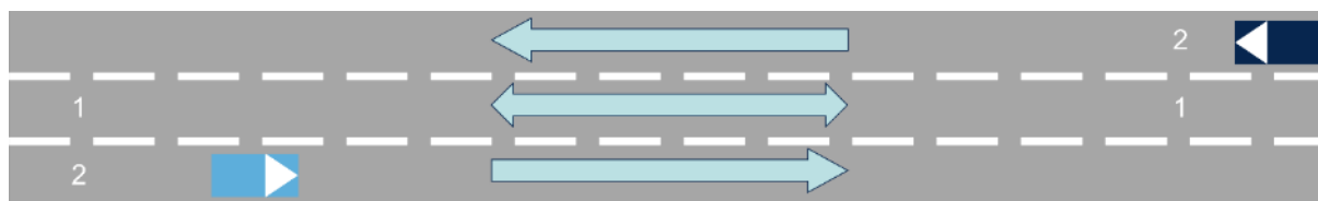
Figure 49: A 3-lane road with the expected ETSI LanePositions . The left numbers are the ETSI LanePositions for vehicles traveling from left to right. The right numbers are the ETSI LanePositions for vehicles travelling from right to left.
